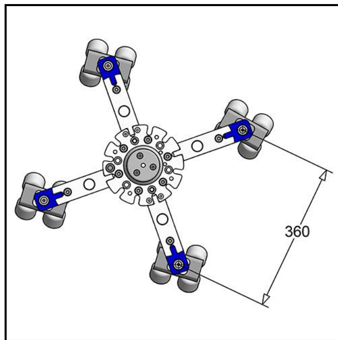
Grip Kit – Small track width (360mm)
