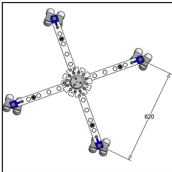
Grip Kit – Normal track width (620mm)
